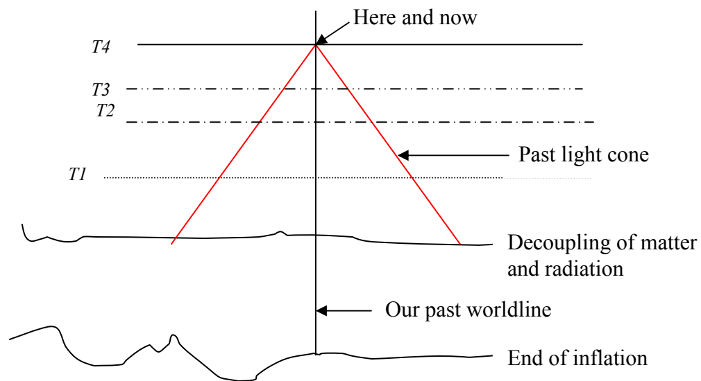
Figure 5: Spacetime diagram of the cosmological context of the development of complexity. Random fluctuations at the end of inflation generated random fluctuations at the surface of decoupling of matter and radiation. First generation stars (without planets) formed at time T1, second generation stars (with planets) at time T2. First life appeared at T3. The present time is T4. The higher level order and meaning at times T3 and T4 is not explicitly coded into the initial data at the end of inflation or at the surface of last scattering. Thus they come into being during the evolution of complex structures; they are allowed by the initial data but not caused by it.
