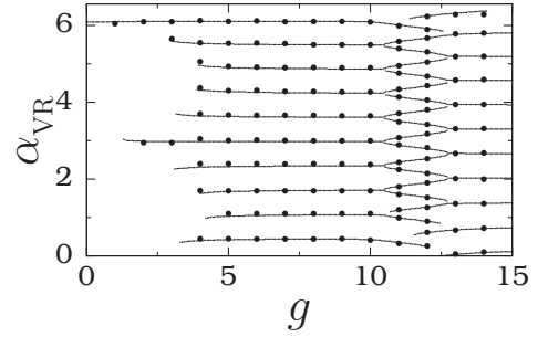
FIG. 11. \alpha_{VR} versus g for the overdamped double-well system with \gamma = -1 . Continuous lines and solid circles represent theoretical and numerical values of \alpha_{VR} , respectively.
