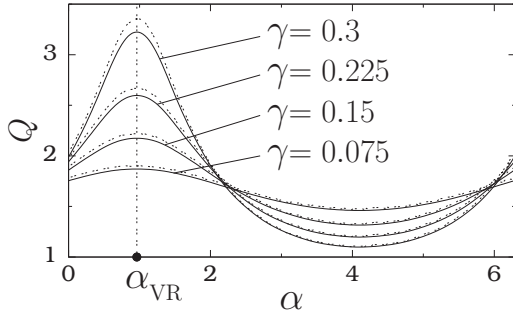
FIG. 9. Response amplitude Q versus the time-delayed parameter \alpha for a few fixed values of \gamma and g = 100 for the underdamped single-well system. The continuous and dashed lines represent theoretically and numerically predicted values of Q , respectively. The vertical dashed line marks the value of \alpha_{\text{VR}} given by Eq. (17).
