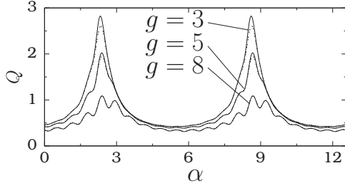
FIG. 16. Response amplitude Q as a function of the delay parameter \alpha for three fixed values of g for the overdamped single-well system. Theoretical and numerical values of Q are represented by continuous and dashed lines, respectively. The dashed lines are not visible for g = 5 and 8 because of the very closeness of theoretical Q with the numerical Q .
