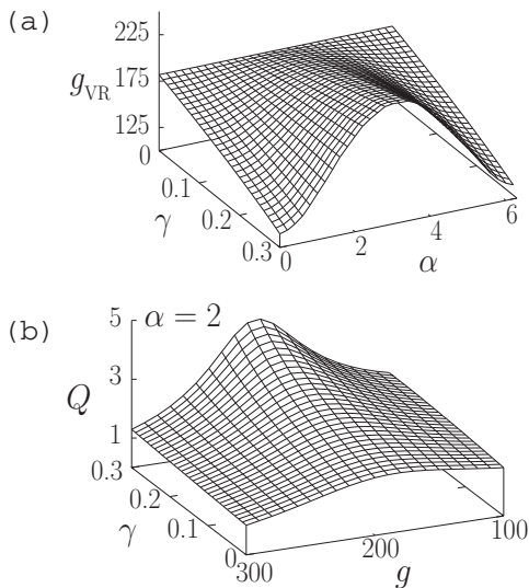
FIG. 7. (a) Theoretical g_{\text{VR}} versus the time-delayed feedback parameters \gamma and \alpha for the underdamped single-well system with \omega_0^2 = 0.5 and \beta = 0.1 . (b) Q versus the parameters \gamma and g for \alpha = 2 .
