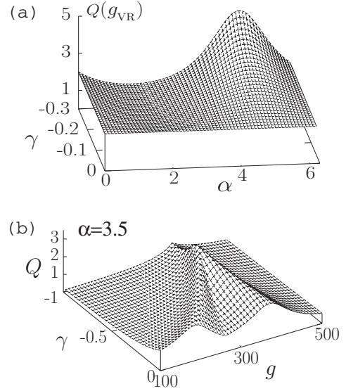
FIG. 3. (a) Variation of the maximum value of Q , Q(g = g_{VR}) , as a function of \gamma and \alpha for the double-well underdamped system. (b) Three-dimensional plot of Q versus the parameters \gamma and g for \alpha = 3.5 .
