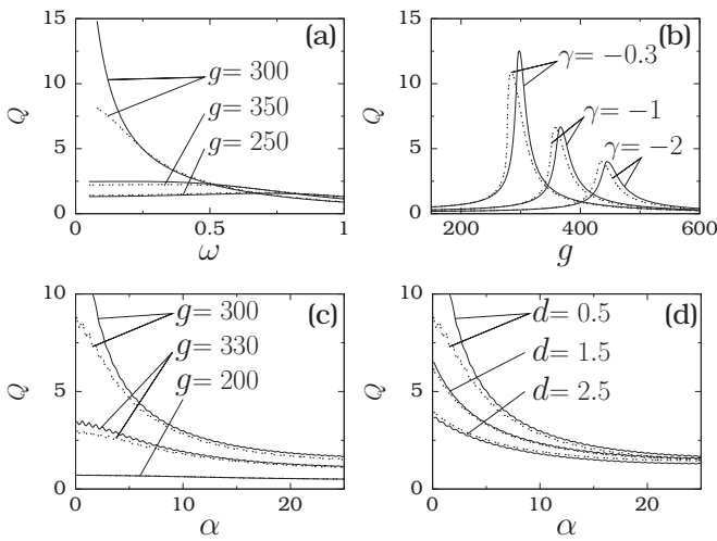
FIG. 17. (a) \omega versus theoretical Q (marked by continuous lines) and numerical Q (marked by dashed lines) for three values of g for system (1) with double-well potential. Here d = 0.5 , \omega_0^2 = -1 , \beta = 0.1 , \gamma = -0.3 , \alpha = 1 , \Omega = 10 , and f = 0.1 . (b) g versus Q for three values of \gamma with \omega = 0.1 . [(c),(d)] \alpha versus Q . (c) \omega = 0.1 , \gamma = -0.3 , and d = 0.5 . (d) \omega = 0.1 , \gamma = -0.3 , and g = 300 .
