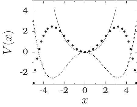
FIG. 1. Single-well (represented by a continuous line, \omega_0^2 = 0.5 , \beta = 0.1 ), double-well (represented by a dashed line, \omega_0^2 = -1 , \beta = 0.1 ), and single-well with double-hump (represented by solid circles, \omega_0^2 = 1 , \beta = -0.1 ) forms of the potential V(x) = \frac{1}{2}\omega_0^2 x^2 + \frac{1}{4}\beta x^4 .
