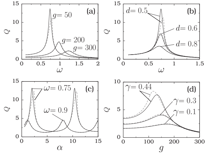
FIG. 18. (a) \omega versus theoretical Q (marked by continuous lines) and numerical Q (marked by dashed lines) for three values of g for the system (1) with a single-well potential. Here d = 0.5 , \omega_0^2 = 0.5 , \beta = 0.1 , \gamma = 0.3 , \alpha = 1 , \Omega = 10 , and f = 0.1 . (b) \omega versus Q for three values of d with g = 50 . (c) \alpha versus Q for two values of \omega with g = 50 and d = 0.5 . (d) g versus Q for three values of \gamma with \alpha = 1 , \omega = 1 , and d = 0.5 .
