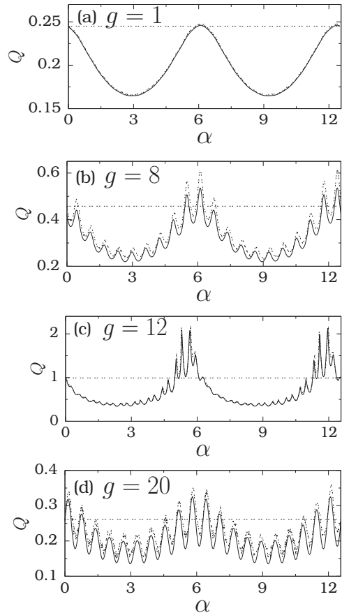
FIG. 12. Theoretical (represented by continuous lines) and numerical (represented by dashed lines) Q as a function of the delay parameter \alpha for four fixed values of the parameter g . The system is the double-well overdamped system with \gamma = -1 . The horizontal dashed line denotes the value of Q in the absence of time-delayed feedback.
