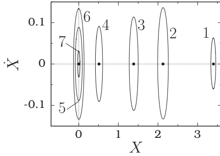
FIG. 4. Phase portraits of the slow motion of the underdamped double-well system for several values of g . The values of g for the numbers 1–7 are 100 (1), 240.5 (2), 275 (3), 295 (4), 300 (5), 376.85 (6), and 600 (7). The values of other parameters are d = 0.5 , \omega_0^2 = -1 , \beta = 0.1 , \gamma = -0.3 , \alpha = 1 , f = 0.1 , \omega = 1 , and \Omega = 10 . The solid circles mark the equilibrium points X_0^* and X_+^* .
