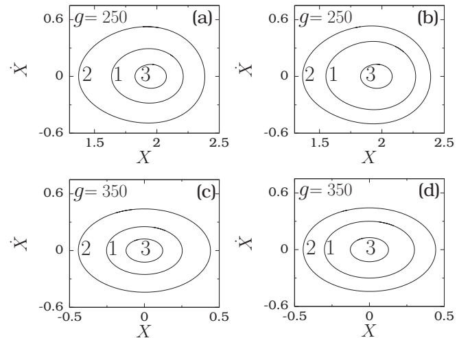
FIG. 6. Phase portraits of the slow orbit as a function of the time-delayed parameter \alpha (\leq 14) for two fixed values of g . (a) g = 250 , \alpha = 4 (1), 4.57 (2), and 8 (3). (b) g = 250 , \alpha = 10.5 (1), 10.97 (2), and 14 (3). (c) g = 350 , \alpha = 3.5 (1), 4.41 (2), and 7 (3). (d) g = 350 , \alpha = 10 (1), 10.69 (2), and 13 (3). In the numerical simulation resonance is observed at \alpha = 4.57 and 10.97 for g = 250 and at \alpha = 4.41 and 10.69 for g = 350 .
