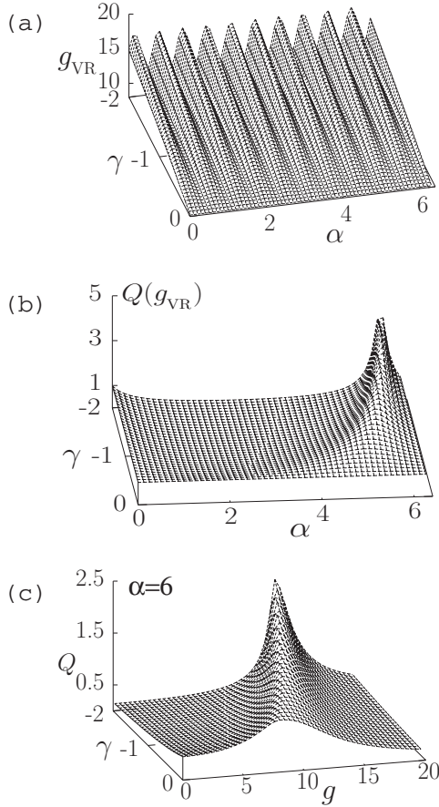
FIG. 10. Theoretically predicted (a) g_{VR} as a function of \gamma and \alpha for the overdamped double-well system with \omega_0^2 = -1 , \beta = 1 , f = 0.1 , \omega = 1 , and \Omega = 10 , (b) Q(g_{VR}) versus the parameters \gamma and \alpha , and (c) variation of the response amplitude Q with \gamma and g for \alpha = 6 .
