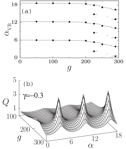
FIG. 5. (a) \alpha_{VR} versus the amplitude g of the high frequency force for \gamma = -0.3 . The system is the underdamped double-well system. Continuous lines and solid circles represent theoretically and numerically computed values of \alpha_{VR} , respectively. (b) Periodic variation of the response amplitude Q with the time-delayed parameter \alpha for various values of g in the interval [100, 300] for \gamma = -0.3 .
