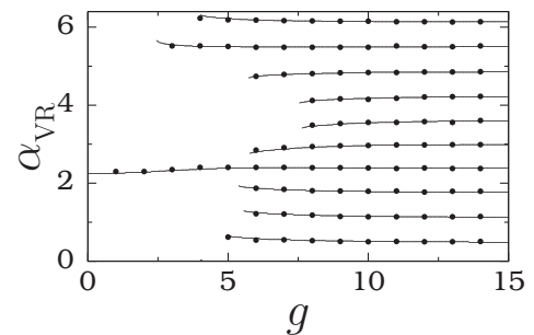
FIG. 15. Plot of theoretical \alpha_{\text{VR}} (represented by continuous lines) and numerical \alpha_{\text{VR}} (solid circles) versus g for \gamma = 1 . The system is the single-well overdamped system.
