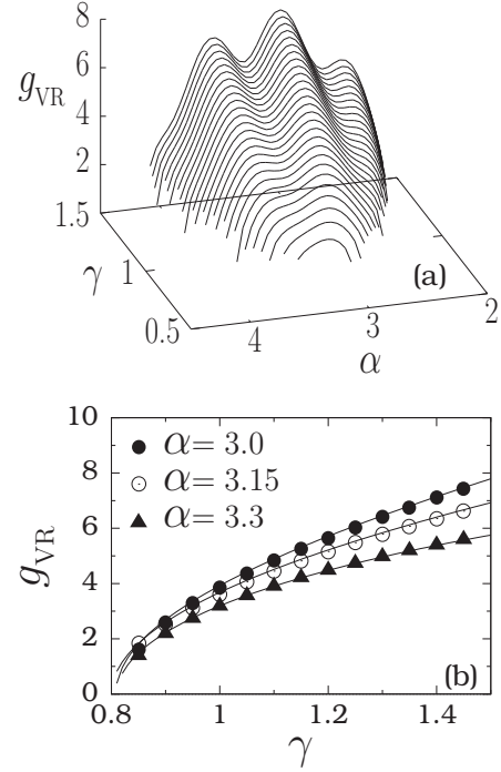
FIG. 14. (a) Theoretically predicted g_{\text{VR}} versus the delay parameters \gamma and \alpha for the single-well overdamped system. The values of other parameters are \omega_0^2 = 0.8 , \beta = 1 , f = 0.1 , \omega = 1 , and \Omega = 10 . (b) g_{\text{VR}} versus \gamma for three fixed values of \alpha . Continuous lines are theoretical g_{\text{VR}} , while the symbols represent numerically computed values of g_{\text{VR}} .
