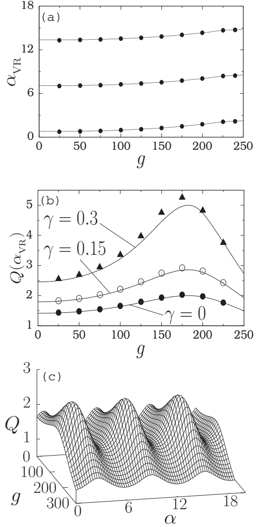
FIG. 8. (a) \alpha_{\text{VR}} versus g for \gamma = 0.15 . The system is the underdamped single-well system. Continuous lines and solid circles represent theoretically predicted and numerically calculated values of \alpha_{\text{VR}} , respectively. Here d = 0.5 , \omega_0^2 = 0.5 , \beta = 0.1 , \gamma = 0.15 , f = 0.1 , \omega = 1 , and \Omega = 10 . (b) Variation of Q(\alpha_{\text{VR}}) with g for \gamma = 0.15 and 0.3 . Q versus g for \gamma = 0 is also shown. The continuous lines and symbols represent theoretically and numerically predicted values of Q . (c) Periodic variation of Q with the time-delayed parameter \alpha for various values of g for \gamma = 0.15 .
