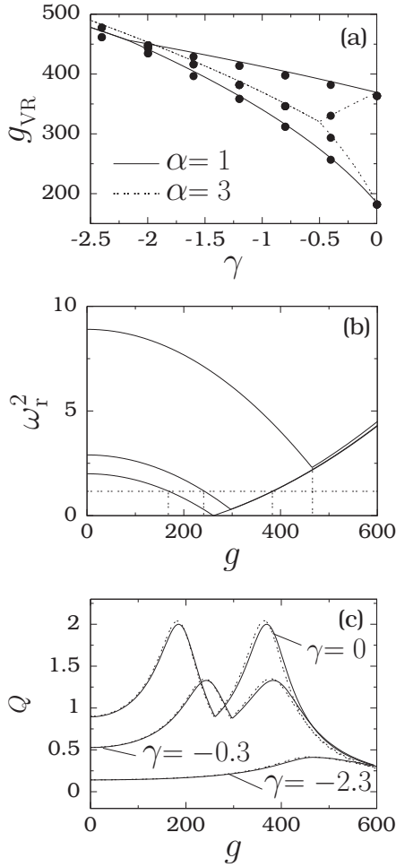
FIG. 2. (a) Theoretical and numerical g_{VR} versus the parameter \gamma for two fixed values of the time-delayed parameter \alpha for the underdamped system (1) with the double-well potential case. The solid circles are the numerically computed g_{VR} and the lines are theoretical g_{VR} . The values of the parameters are d = 0.5 , \omega_0^2 = -1 , \beta = 0.1 , f = 0.1 , \omega = 1 , and \Omega = 10 . (b) The variation of theoretical \omega_r^2 with parameter g . From bottom to top, the curves show the values of \gamma are 0, -0.3 , and -2.3 , respectively. The horizontal dashed line represents the value of (\omega^2 - \gamma \cos \omega \alpha) . The vertical dashed lines mark the values of g_{VR} . (c) Plot of the response amplitude Q as a function of g for \gamma = 0, -0.3 , and -2.3 with \alpha = 1 . The continuous lines are theoretical Q , while the dashed lines are numerically calculated Q .
