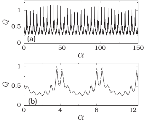
FIG. 13. (a) Quasiperiodic variation of Q with the delay parameter \alpha for \omega = \sqrt{2} , \Omega = 10 , and g = 10 . The system is the overdamped double-well system. (b) Enlargement of part (a). Continuous and dashed lines represent the theoretically and numerically calculated values of Q , respectively.
