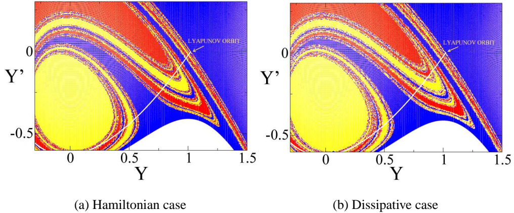
FIG. 11: For E = 0.25 in the Hénon-Heiles system, a segment of the unstable manifold of one of the three Lyapunov orbits, an unstable periodic orbit accessible to at least one basin. That the segment intersects all four basins suggests the Wada property of the basins, (a) in the Hamiltonian case, (b) in the dissipative case with \alpha = 10^{-4} , and \beta = 10^{-4} .
