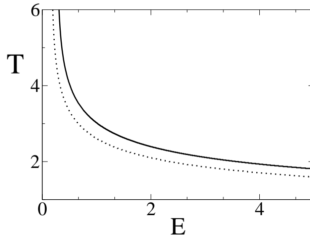
FIG. 3: Average delay time versus the energy. The time diverges as the particle energy approaches the threshold value E_e from above. (a) Dotted curve is for non-dissipative case. (b) Solid curve is for dissipative case with \alpha = \beta = 10^{-3} .
