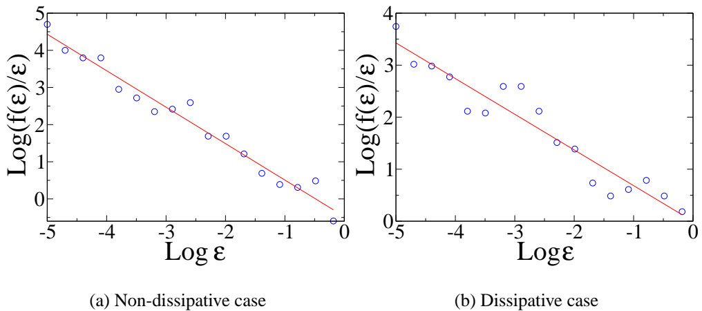
FIG. 6: For E = 0.19 in the Hénon-Heiles system so that there is chaotic scattering, algebraic scaling of f(\epsilon)/\epsilon with \epsilon . The absolute value of the slope from a linear fit gives the a good estimate for the fractal dimension of the set of singularities in the delay-time function. We obtain D = 0.97 \pm 0.01 for the conservative case and D = 0.71 \pm 0.02 for the weakly dissipative case.
