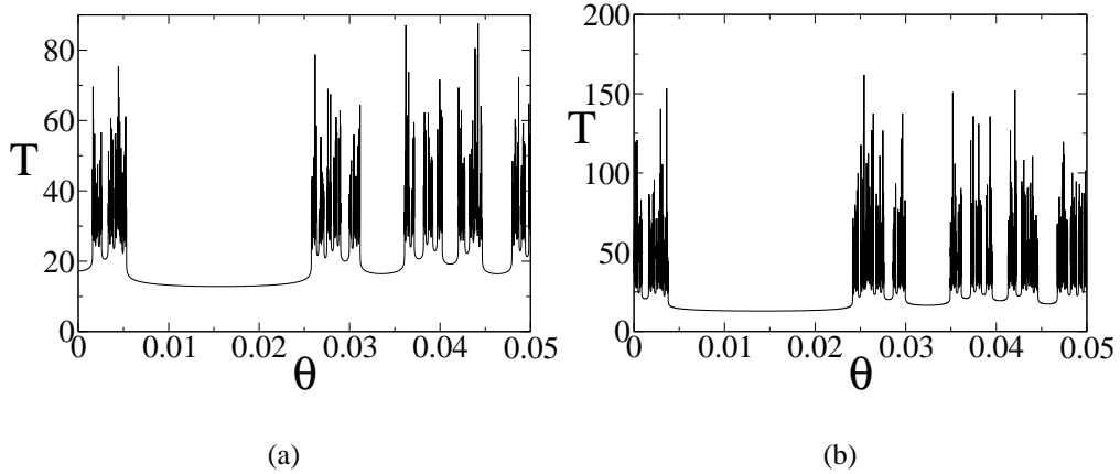
FIG. 5: Typical delay-time function for the conservative (a) and the weakly dissipative (b) Hénon-Heiles system with chaotic scattering ( E = 0.19 , \alpha = 10^{-4} , and \beta = 10^{-4} ).
