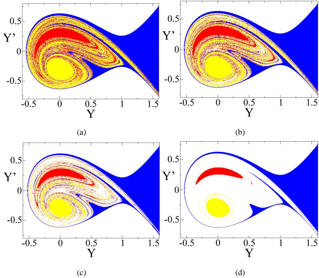
FIG. 9: (a-d) Basins of scattering destinations and of the fixed-point attractor at the center of the scattering region for E = 0.19 and for \mu = 5 \times 10^{-4} , 10^{-3} , 10^{-2} , and 10^{-1} , respectively.
