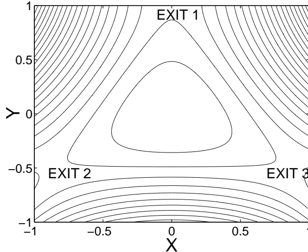
FIG. 1: Representative contours of the Hénon-Heiles potential. Closed curves correspond to energy E < E_e = 1/6 . There are three symmetric destinations for scattering particles.
