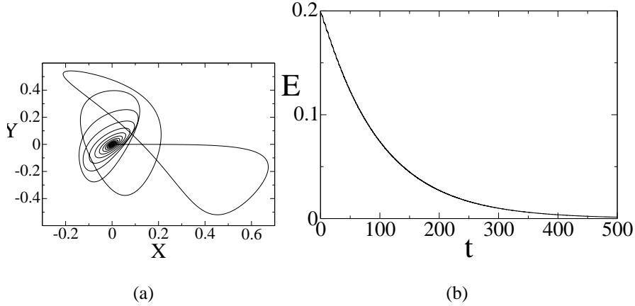
FIG. 4: (a) In the presence of dissipation ( \alpha = 0.1 and \beta = 0.1 ), a particle permanently trapped in the scattering region. The corresponding trajectory approaches the fixed-point attractor in the phase space. (b) Exponential decay to zero of the particle energy when it approaches the attractor.
