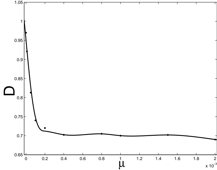
FIG. 7: The uncertainty dimension D versus the dissipation parameter \mu = \alpha = \beta . The rapid decrease in D for \mu \gtrsim 0 is characteristic of a cusp.
