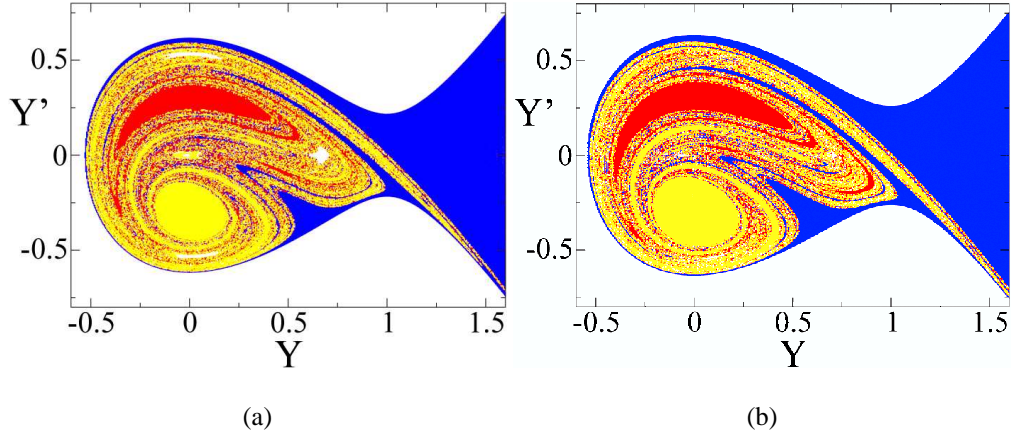
FIG. 8: For E = 0.19 in the Hénon-Heiles system, (a) the basins of scattering particles in the conservative case. In this case, there are three destinations, and initial conditions going to the destinations are distinguished by three colors and the white regions inside the plotted structure denote the KAM islands. (b) The basin structure in the presence of a small amount of dissipation ( \alpha = 10^{-4} and \beta = 10^{-4} ). Due to the dissipation, an additional destination arises: the fixed-point at the center of the scattering region. Four colors are then needed to distinguish the initial conditions. See text for simulation details.
