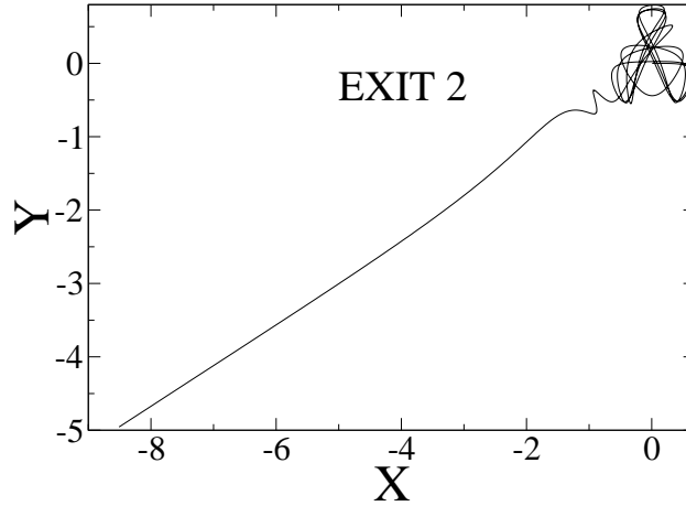
FIG. 2: A typical scattering trajectory in the Hénon-Heiles system with E = 0.2 , where the particle escapes through exit 2 in Fig. 1.
