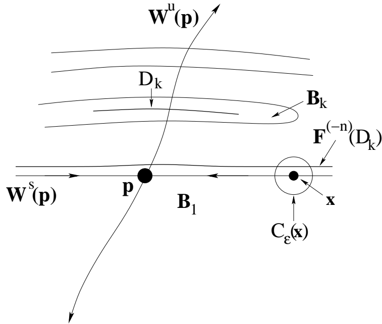
FIG. 10: Schematic illustration of the Kennedy-Yorke theorem establishing the Wada property. See text for details.
